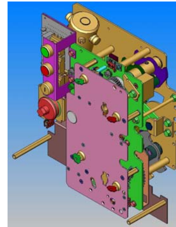
KR Mechanism
